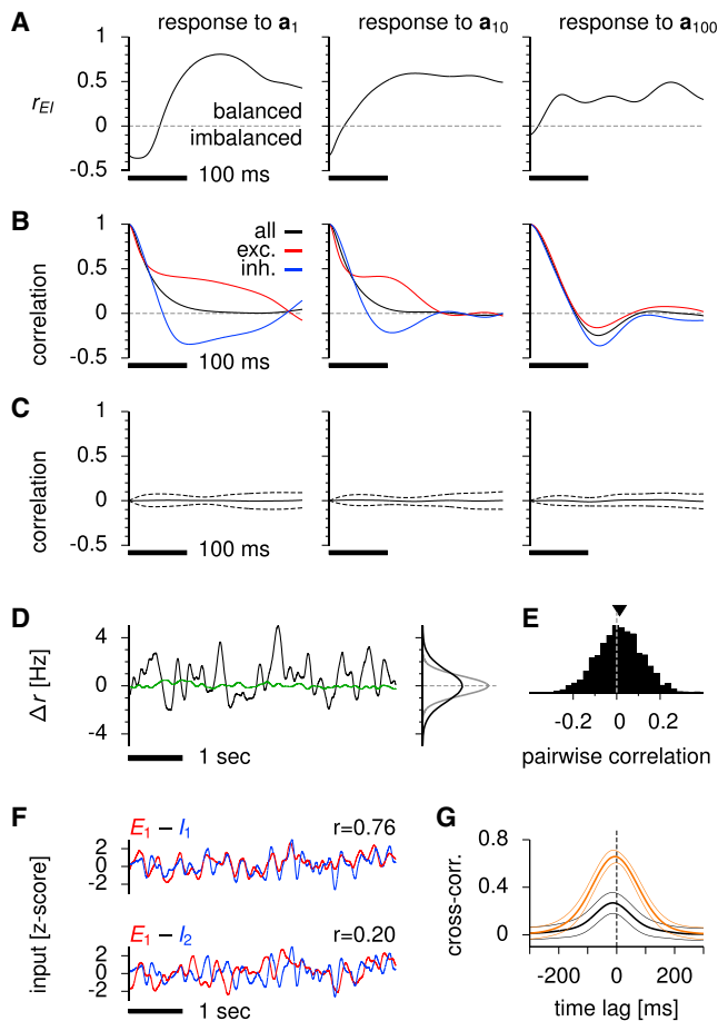
Figure 6. Precise Balance of Excitation and Inhibition in SOC
