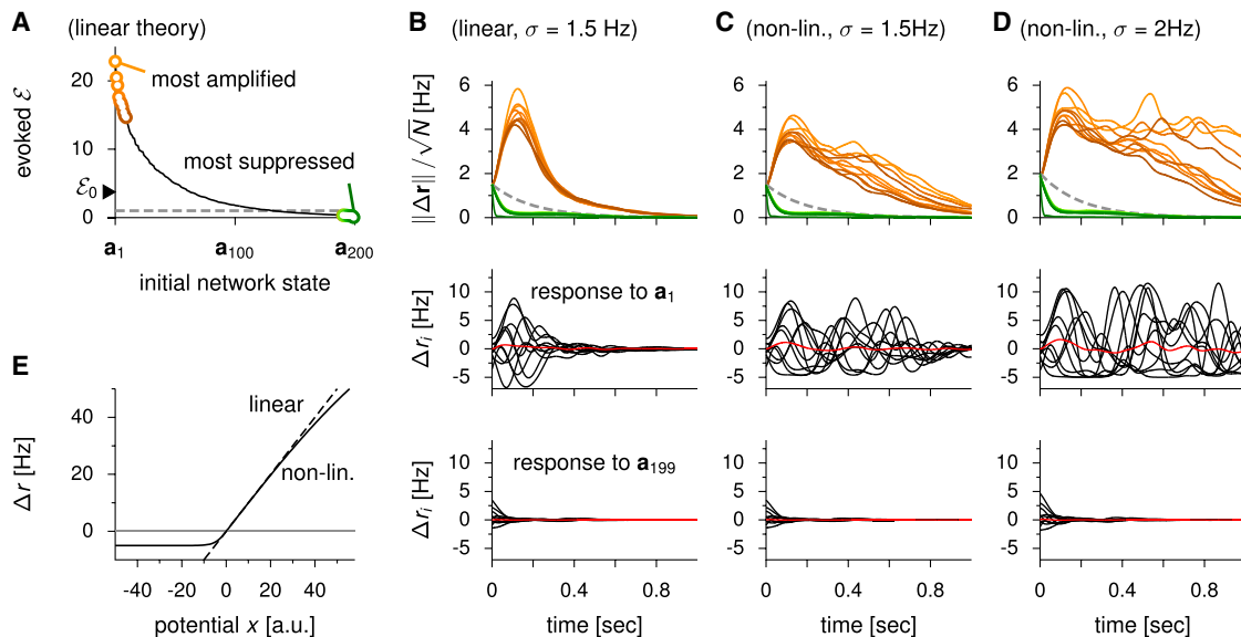
Figure 3. Transient Amplification in SOC
