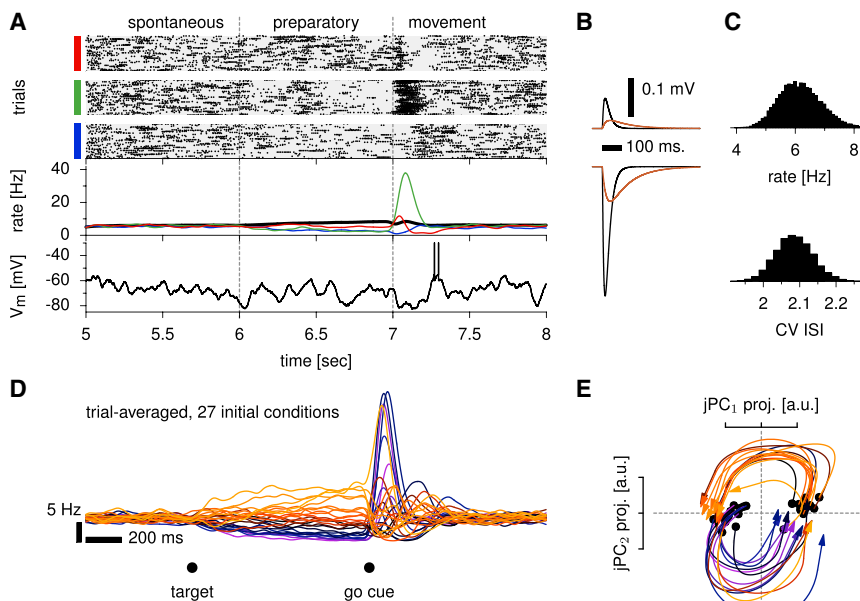
Figure 7. Transient Dynamics in a Spiking SOC
